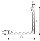
L2 ARSTYL® H 200 x W 250 mm C 30 mm - D 15 mm p33
