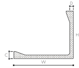
L2 ARSTYL® H 200 x W 250 mm C 30 mm - D 15 mm p33
