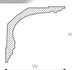
Z7 ARSTYL® H 220 x W 100 mm
